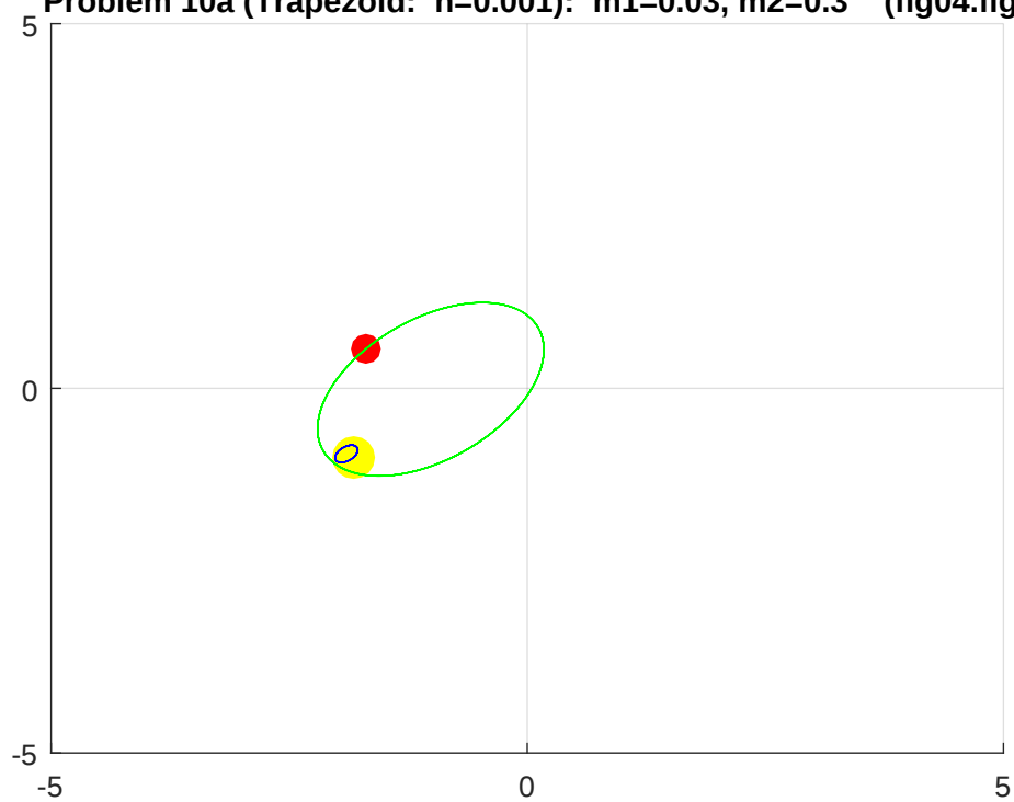
Celestial Mechanics: Two (2) Body Problem Problem 10a (Trapezoid: h=0.001 ): m_1=0.03 , m_2=0.3 (fig04.fig)
